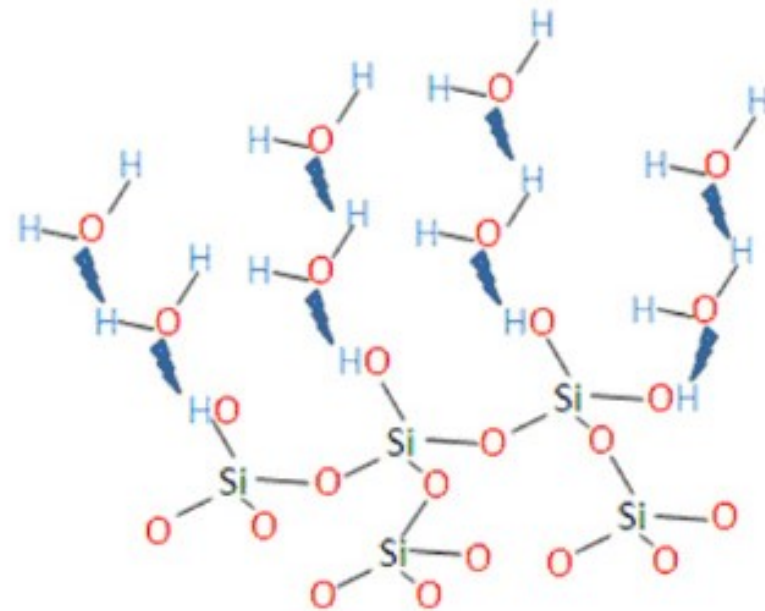
Hydroxylated SiO 2
