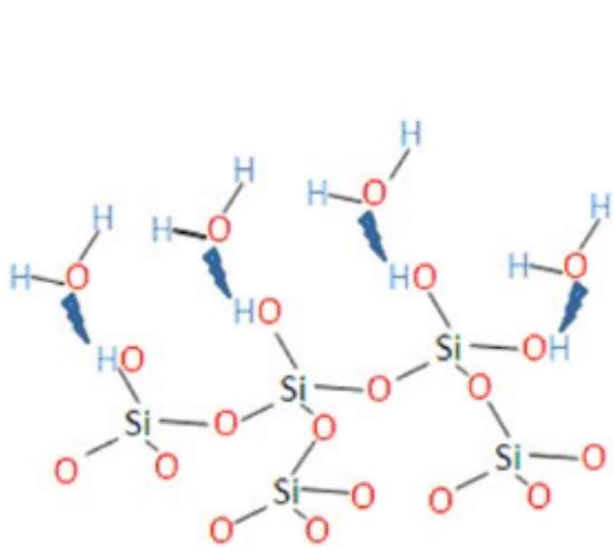
Amorphous SiO 2
