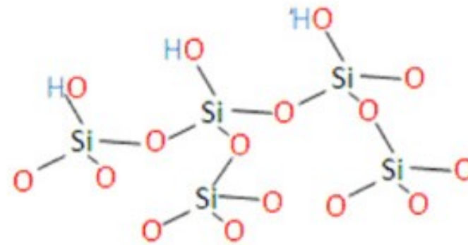
Hydroxylated SiO 2
