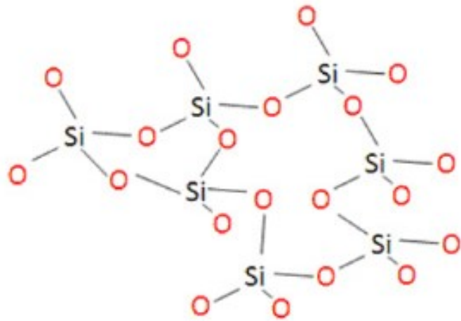
Amorphous SiO 2
